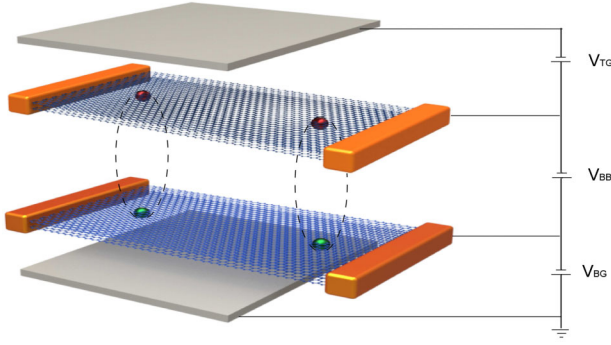
FIG. 1 (color online). Spatially separated electron-hole system (2BLG) with electrons in one graphene bilayer sheet separated by a hBN dielectric barrier from holes in a second graphene bilayer sheet. Top and bottom metal gates control the densities.
